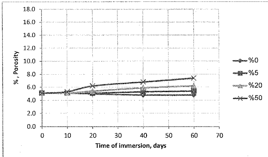
Figure 4.9: Effects of different concentrations of magnesium sulfate on porosity of cement mortar at different ages.
