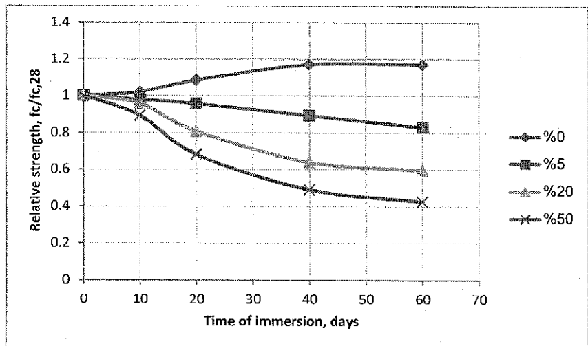
Figure 4. 7: Relative strength of the cement mortar in water and in 5%, 20% and 50% MgSO 4 solutions
