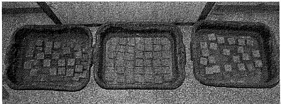
Figure 3.6: Curing of specimens in water tanks.
