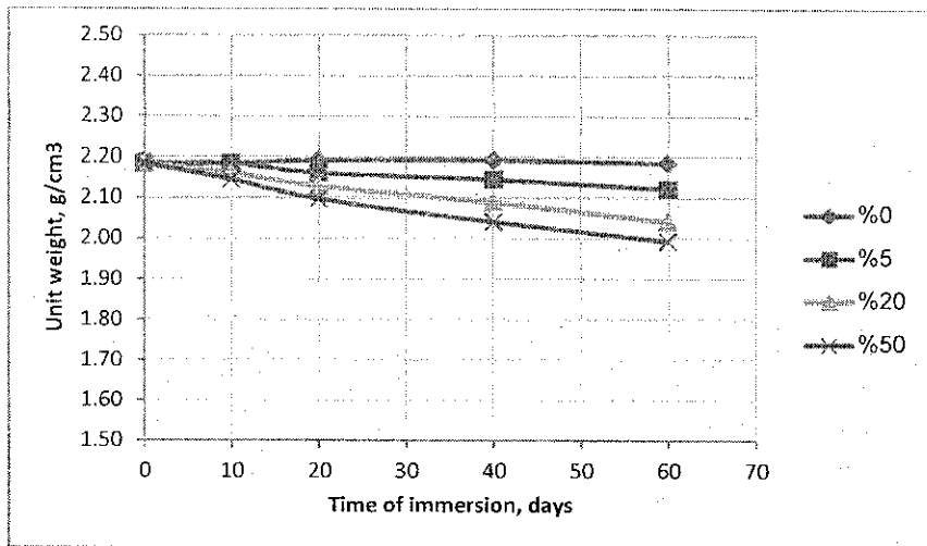
Figure 4. 5: Effects of different concentrations of ammonium nitrate on unit weight of cement mortar at different ages.
