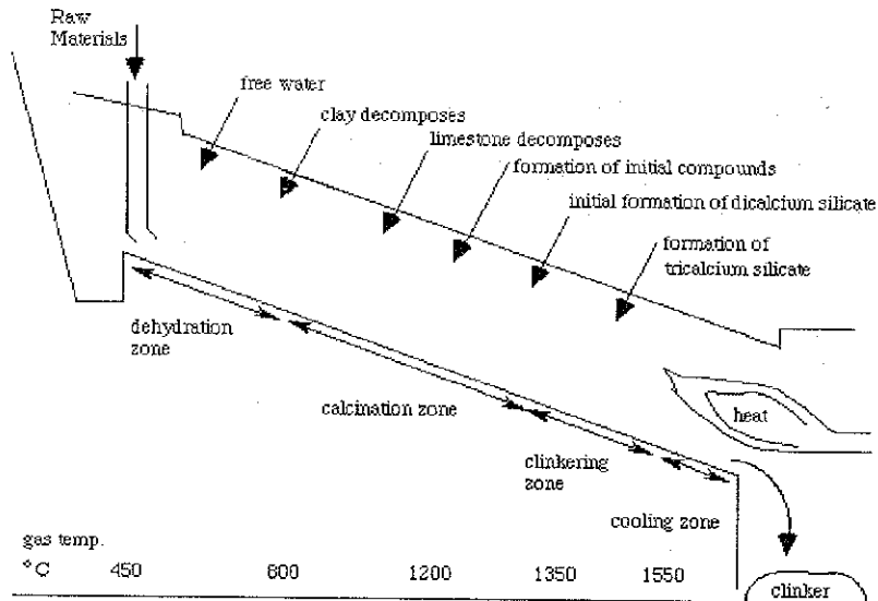
Figure 2.1: Schematic diagram of rotary kiln. (Source: (MAST, 1995))
