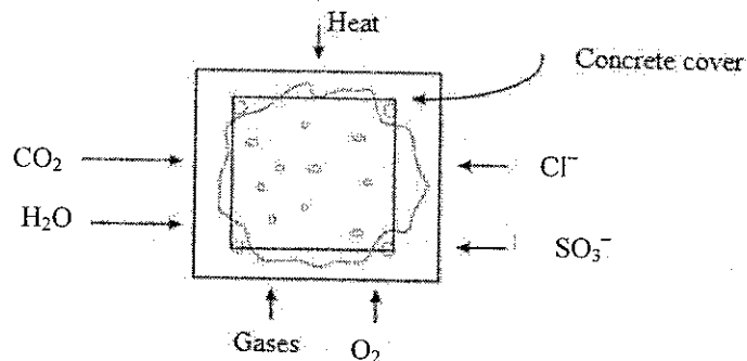
Figure 2.6: Atmospheric agents attacking concrete. (Source: (IRICEN, 2007))
