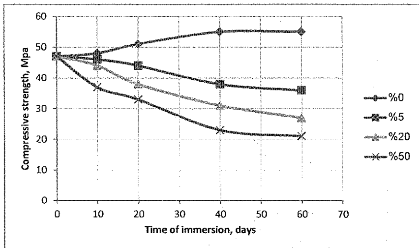
Figure 4.1: Effects of ammonium nitrate on compressive strength of cement mortar at different ages.
