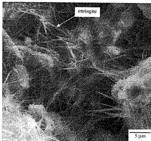
Figure 2. 3: Formation of ettringate within hydrated cement paste. (Source: (Gemelli, Cruz & Camargo, 2004))
