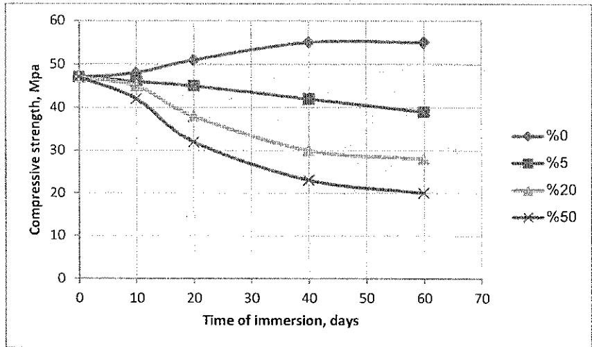
Figure 4.6: Effects magnesium sulfate on compressive strength of cement mortar at different ages.
